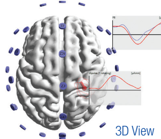
Dipole Clustering
