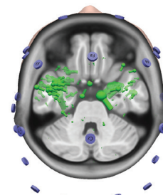
Dipole Clustering
